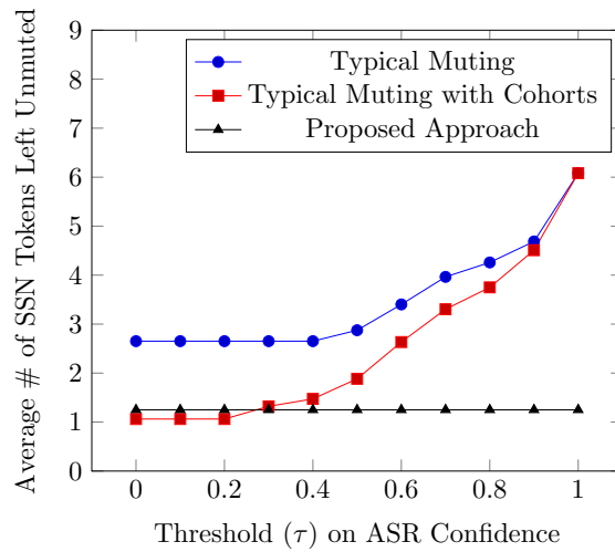
Fig. 4. Comparison of muting approaches. (Proposed Approach comprises fuzzy muting with cohorts.)
