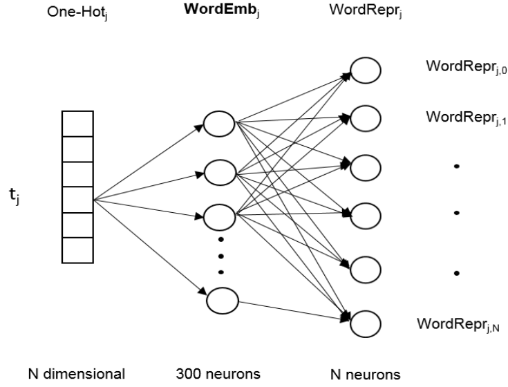
Fig. 1. Neural architecture to generate Word Embedding from Word Representation
