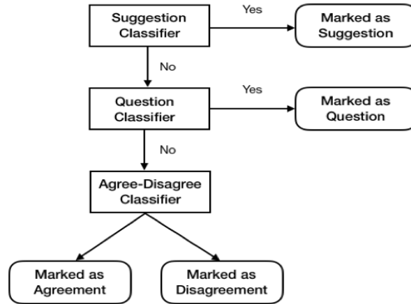
Fig. 1: Hierarchical Classification Workflow
