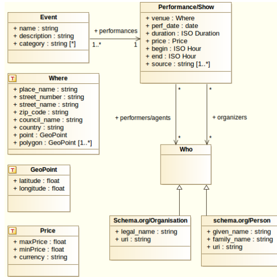
Figure 2. social event representation model
