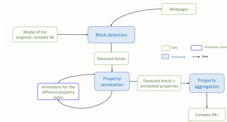
Figure 3. Complex NE general extraction process
